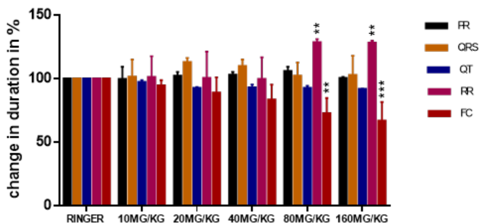
Figure 8. Impacts of hydroethanolic leaf extract of H. bonariensis on electrocardiogram (ECG) waves duration in rabbits. n = 4 . ** p < 0.01 et *** p < 0.001 (ANOVA two ways + dunnetts'test). The extract at 80 mg/kg and 160 mg/kg significantly increased the duration of the RR interval of the ECG, inducing a significant decreased heart rate. The durations of the QT, PR, P-wave, QRS and T-wave intervals were insignificantly impacted by the extract administered in the rabbits.
